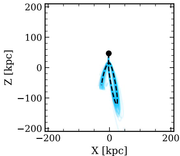
Potential: MWPotential2014 with LMC
