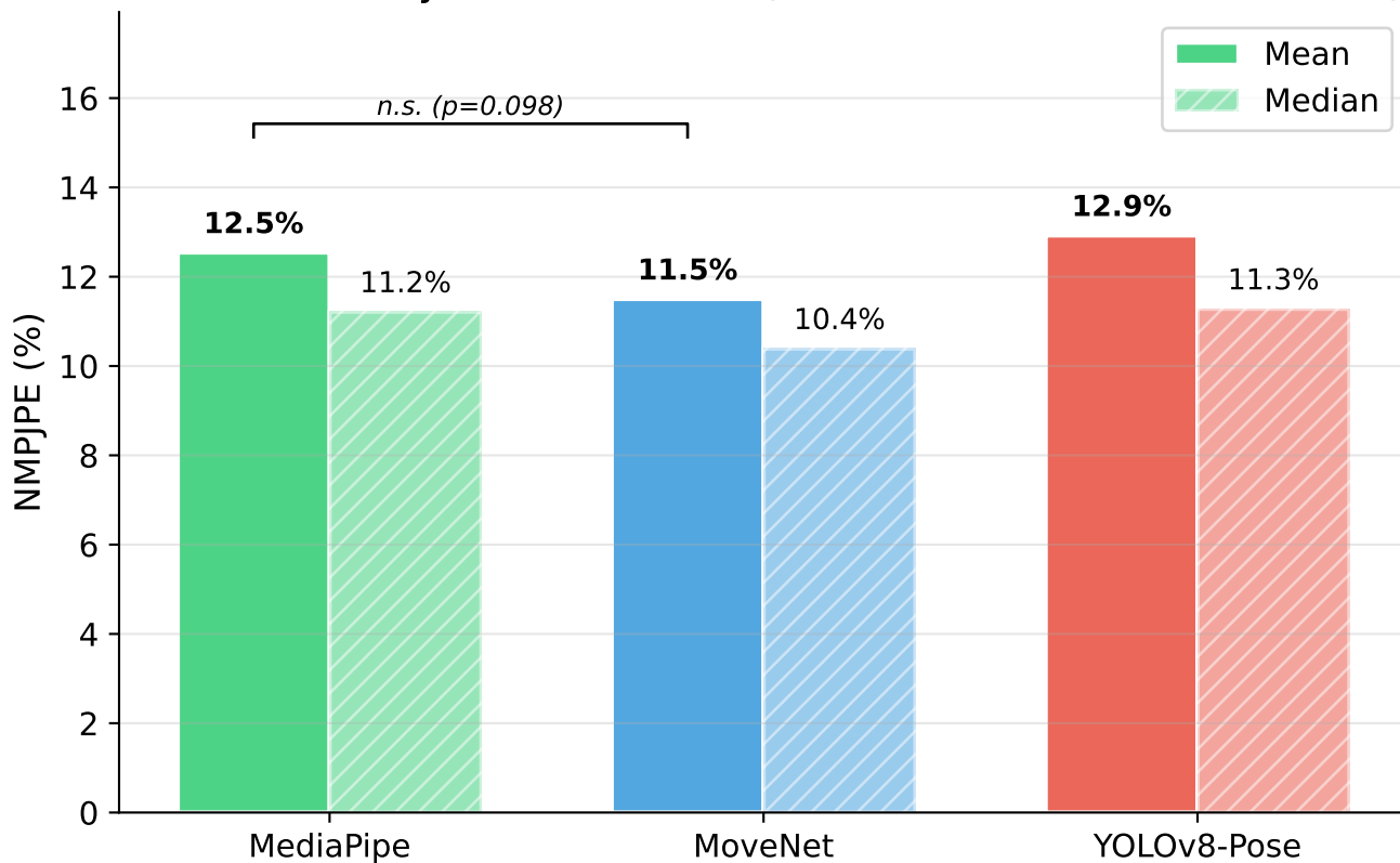
Model Accuracy on REHAB24-6 (Clean Data, Outliers Removed)
