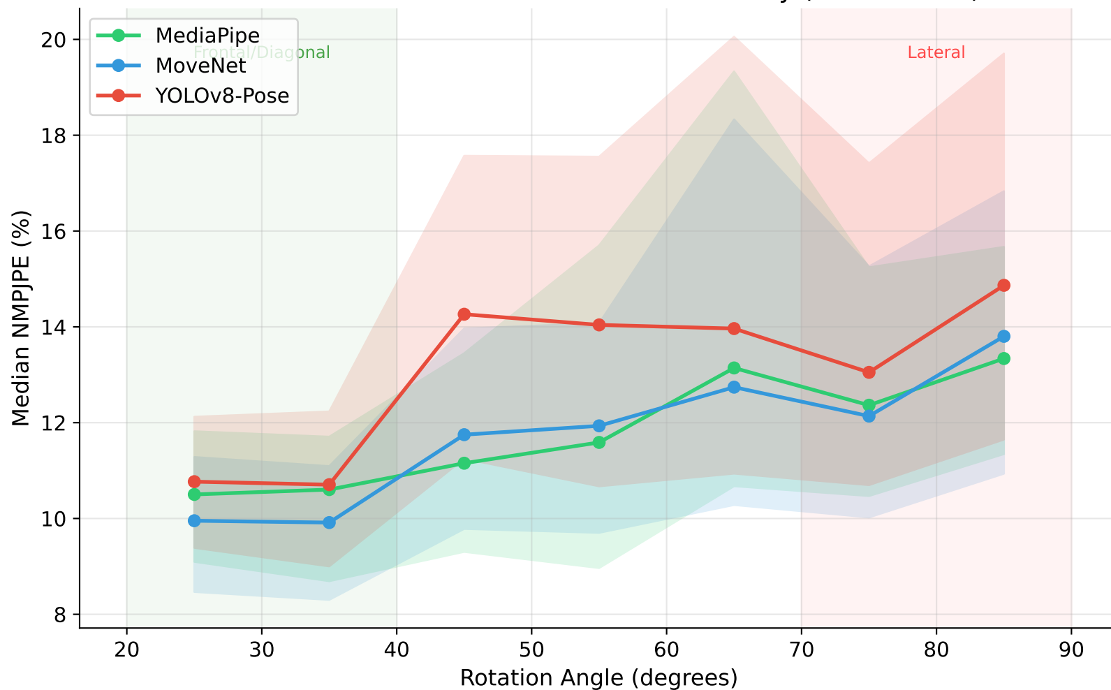
Rotation Effect on Pose Estimation Accuracy (c18 Camera)
