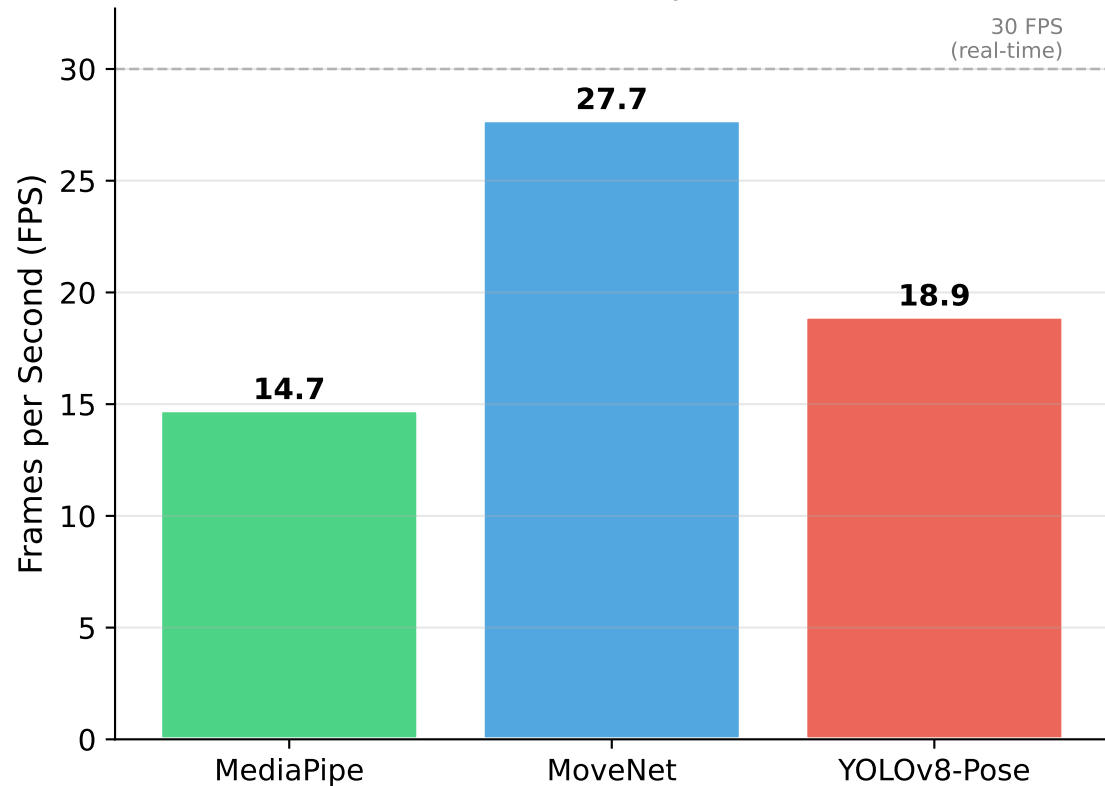
Inference Speed
