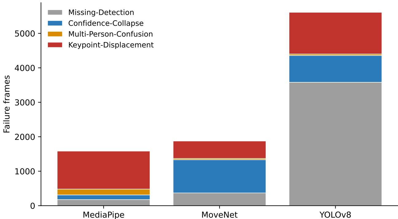
Failure-mode taxonomy by model (REHAB24-6)
