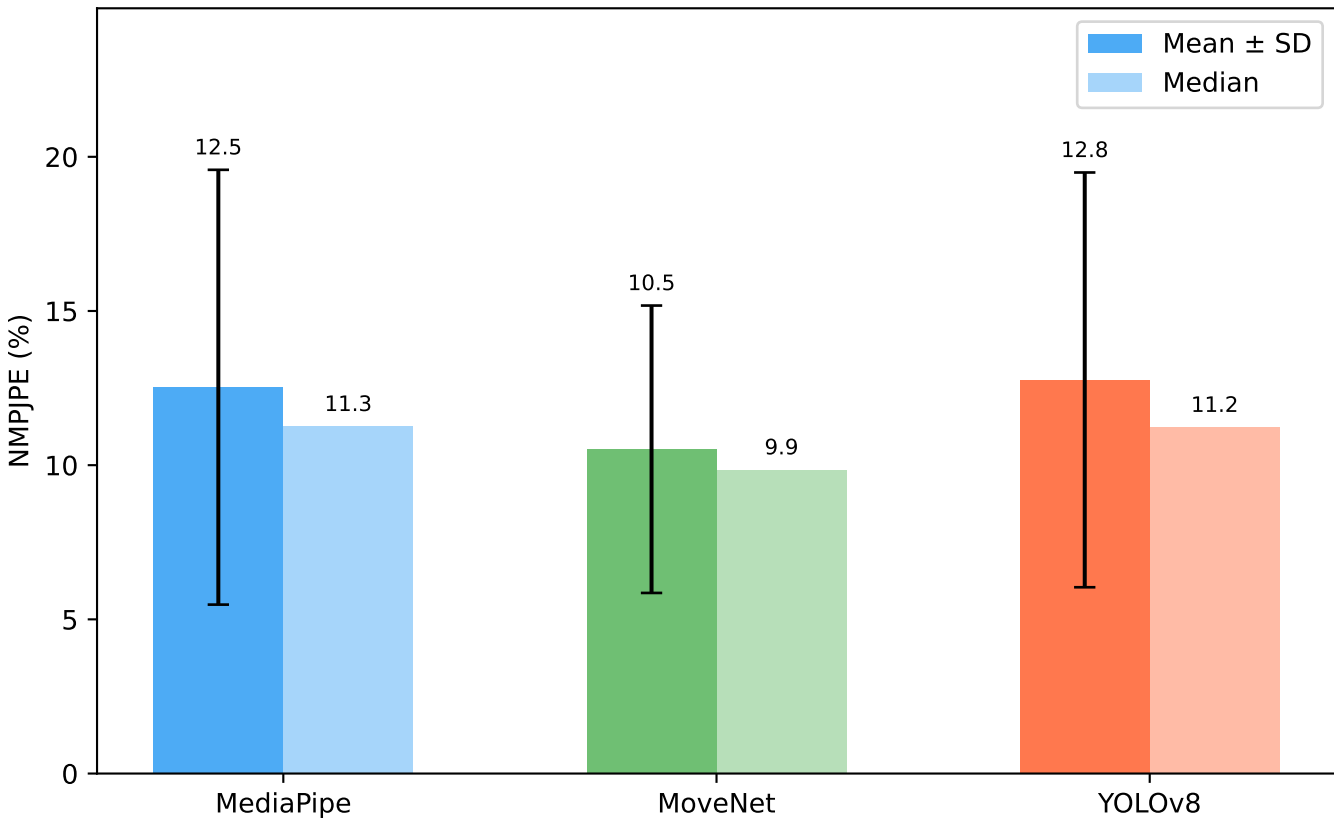
Overall Accuracy (lower is better)
