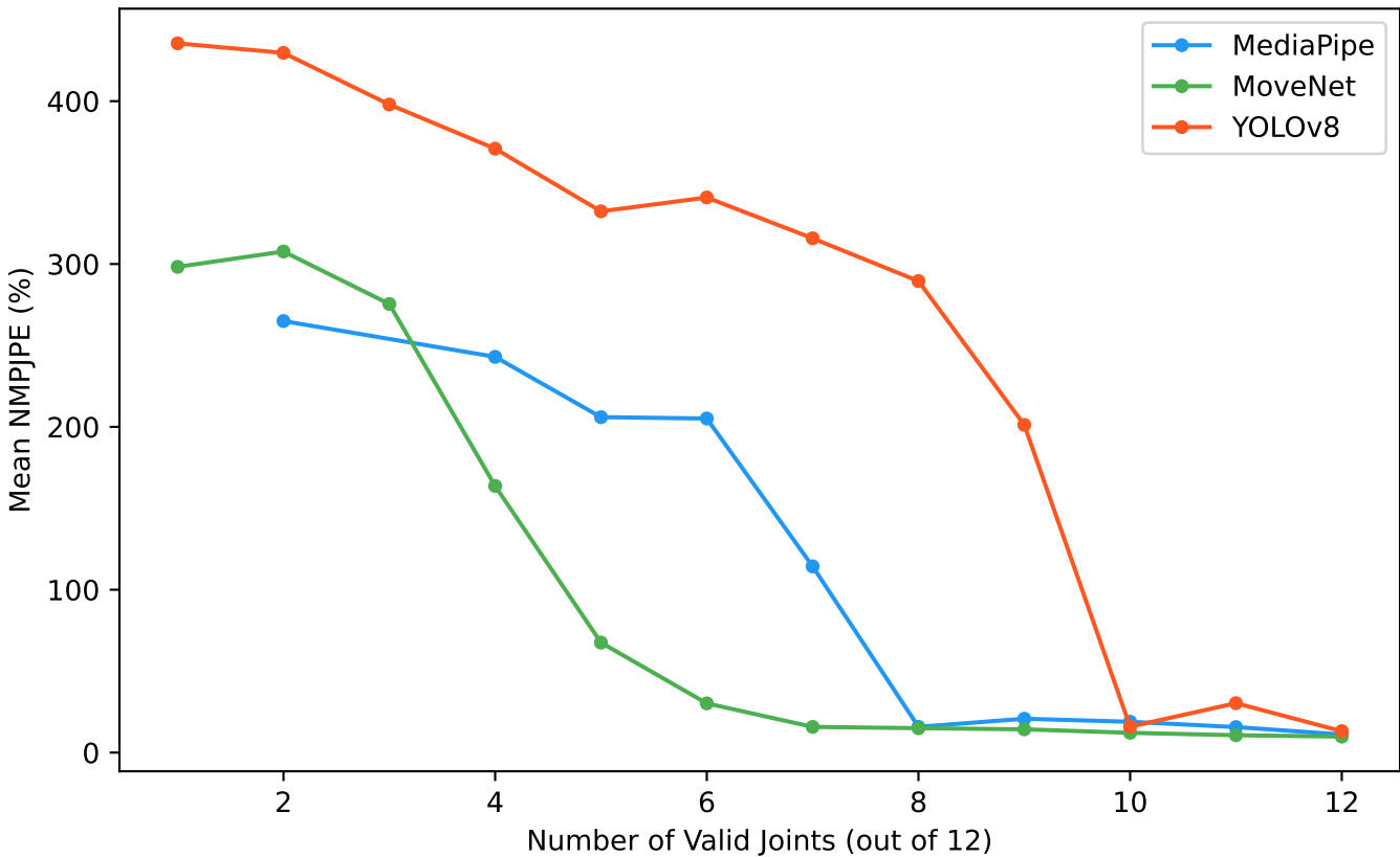
Accuracy vs Detection Completeness
