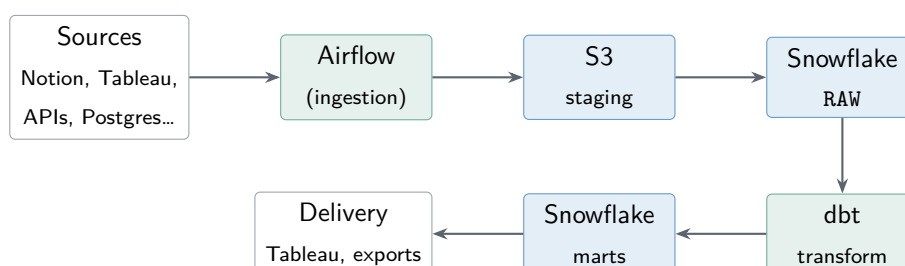
Figure 1.9: Simplified daily ETL chain of the Data Platform.
