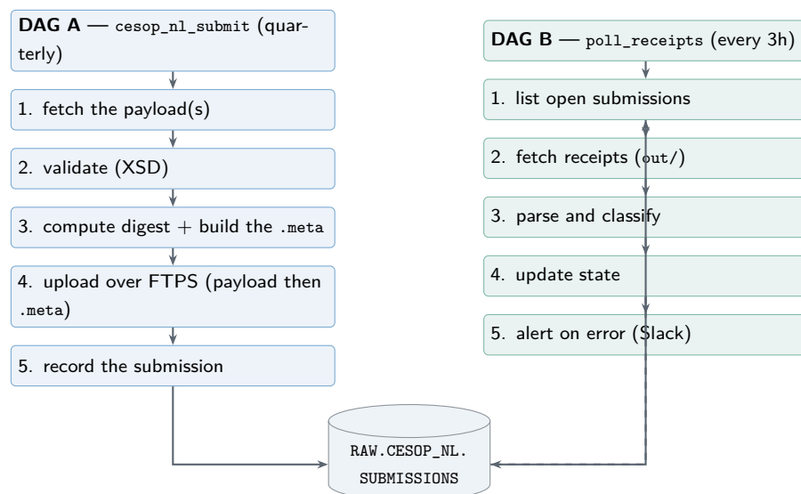
Figure 5.1: CESOP’s Two-DAG architecture: a quarterly submitter and a three-hourly receipt poller, linked by a state table.
