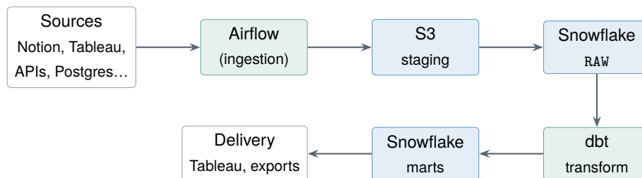
Figure 1.1: Simplified daily ETL chain of the Data Platform.
