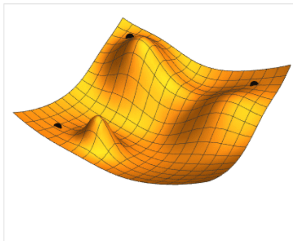
Illustration of gradient descent for three different starting points; two parameters (represented by the plan coordinates) are adjusted in order to minimise the loss function (the height).
