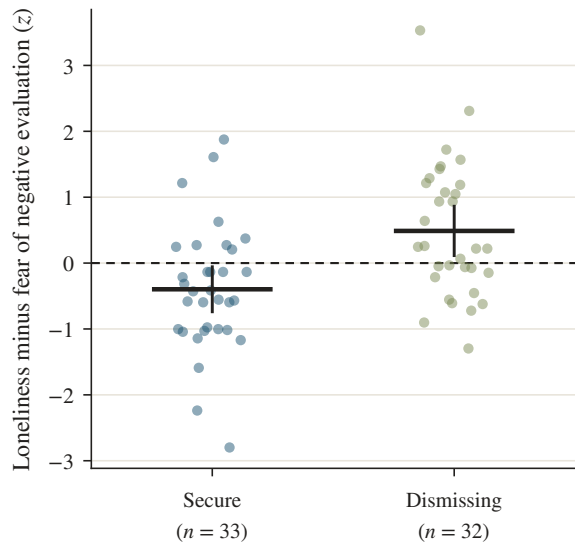
b t = 3.57, p = 0.0007 , Hedges' g = 0.88
