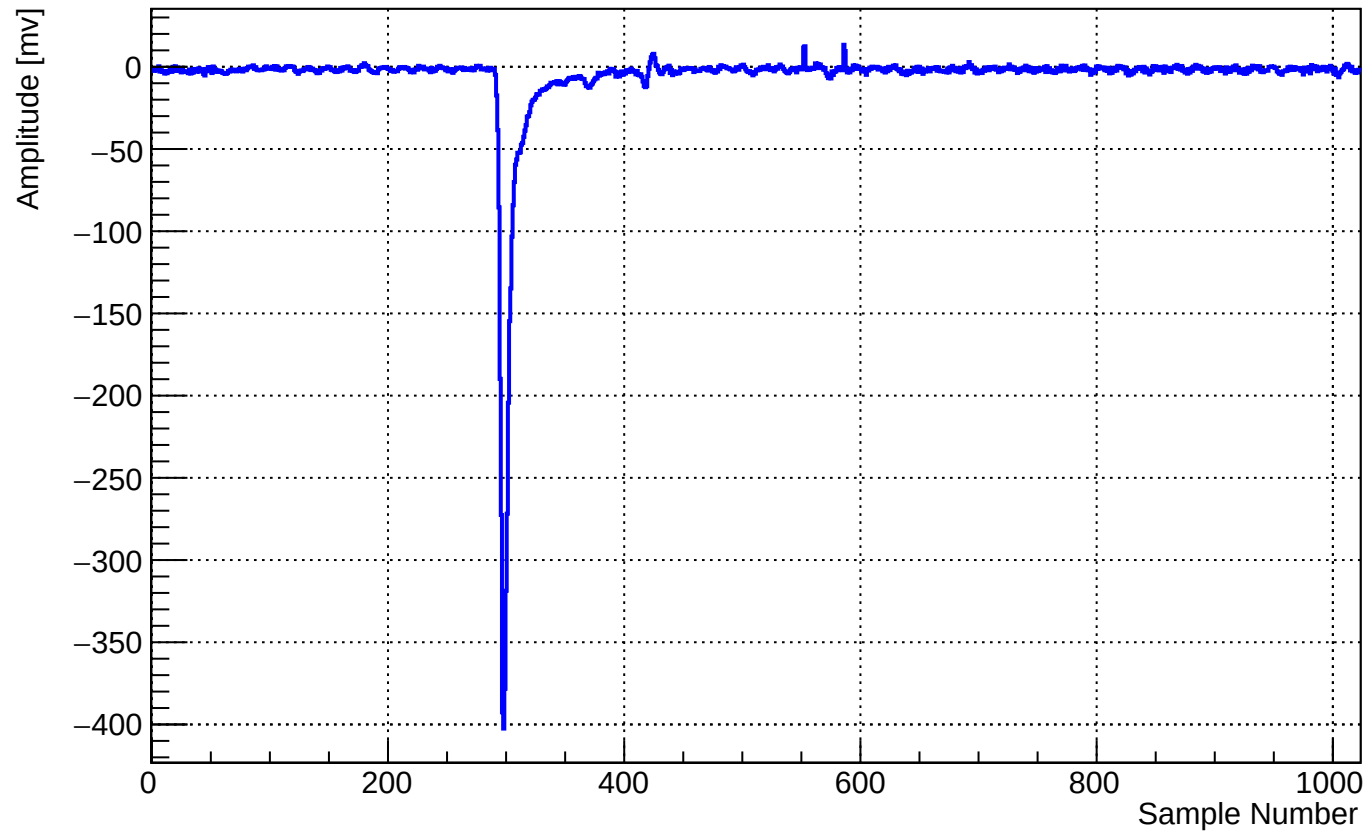
waveform channel 1
