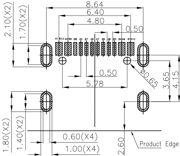
RECOMMENDED P.C.B. LAYOUT TOLERANCE UNSPECIFIED ±0.05mm
