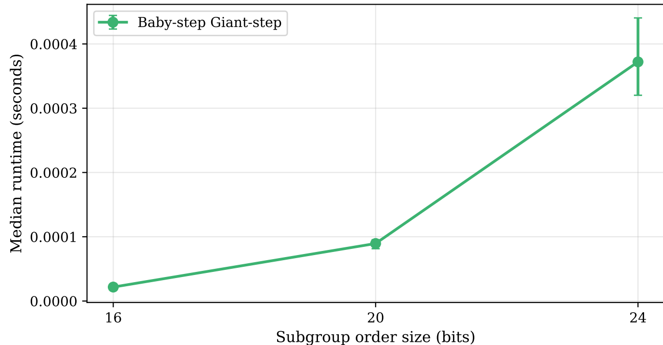
BSGS: Runtime vs. Subgroup Order Size (median of 50 trials, error bars: IQR)
