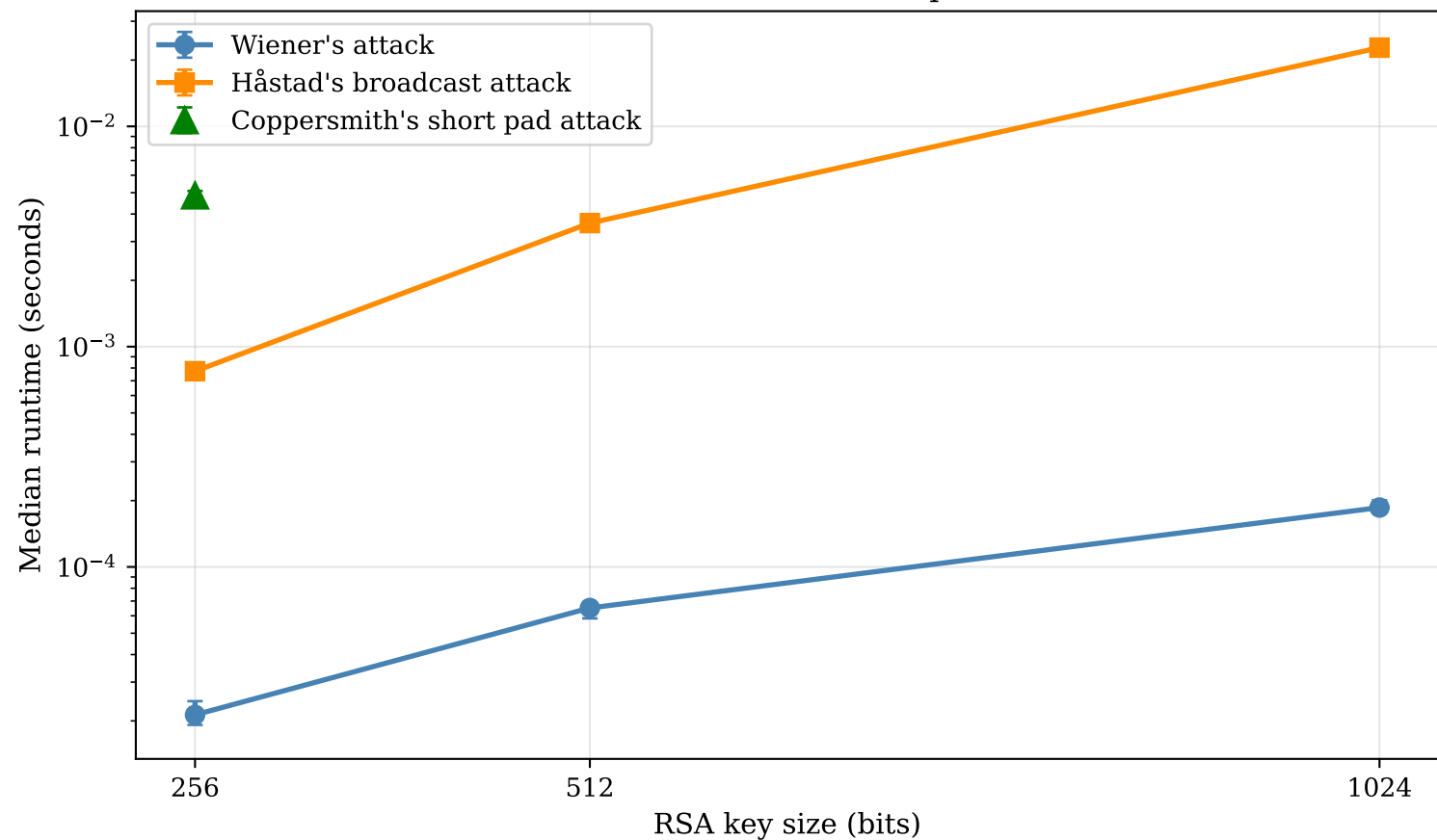
RSA Attack Runtime Comparison
