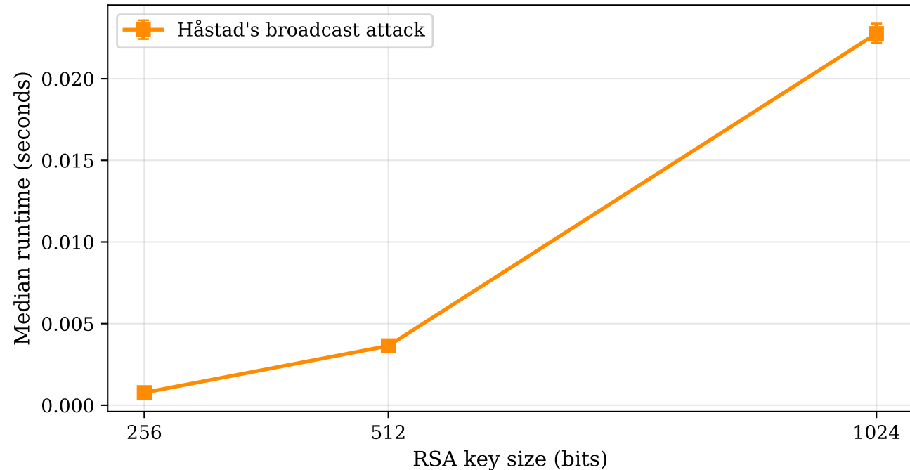
Håstad's Broadcast Attack: Runtime vs. Key Size (median of 50 trials, error bars: IQR)
