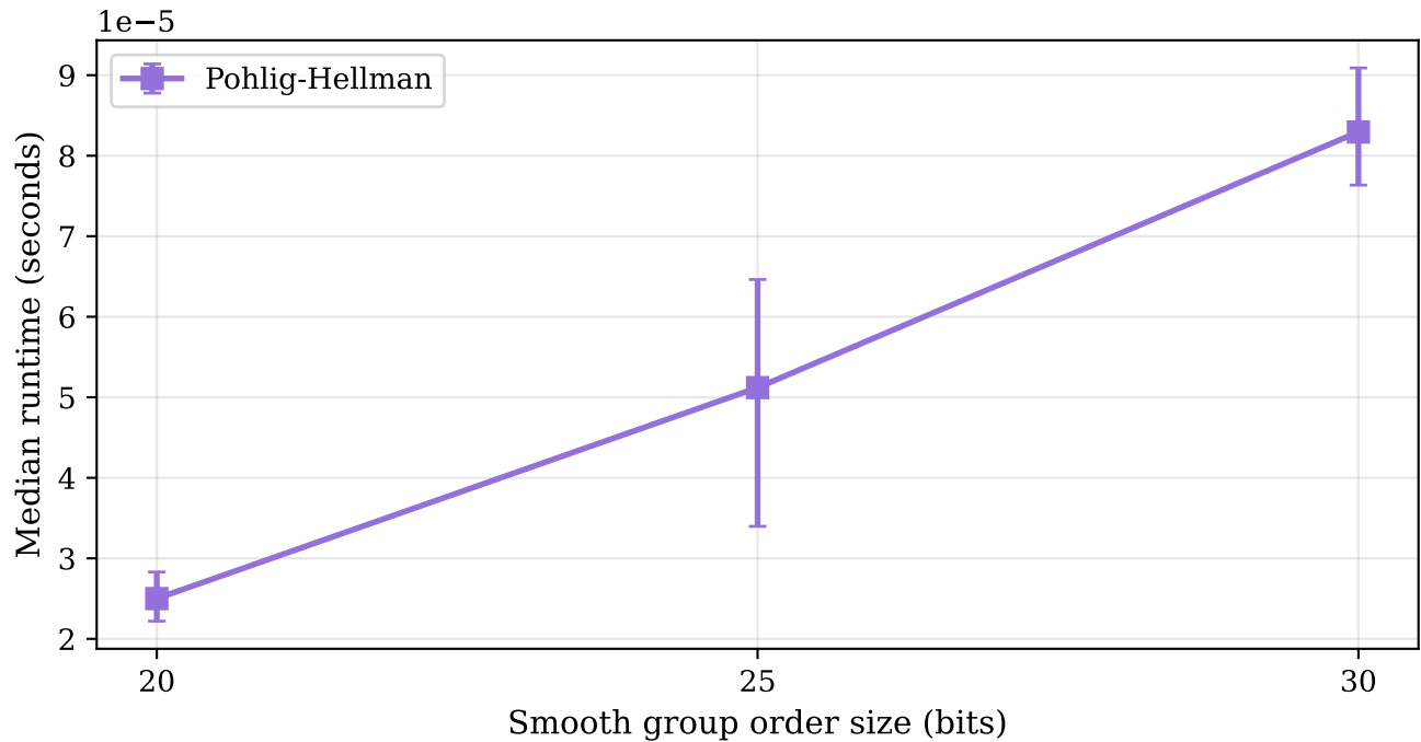
Pohlig-Hellman: Runtime vs. Group Order Size (median of 50 trials, error bars: IQR)
