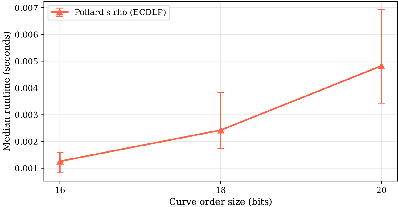
Pollard's Rho (ECDLP): Runtime vs. Curve Order Size (median of 50 trials, error bars: IQR)
