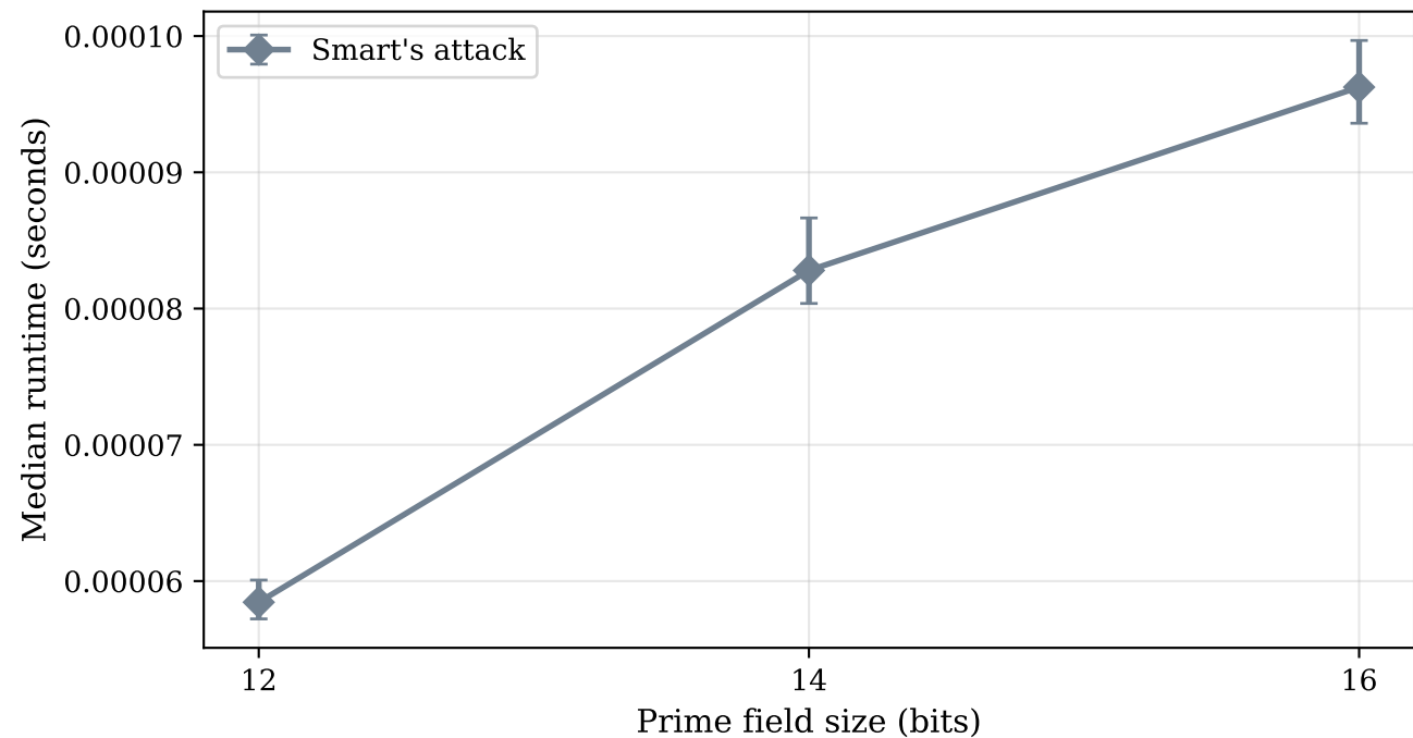
Smart's Attack: Runtime vs. Prime Field Size (median of 50 trials, error bars: IQR)
