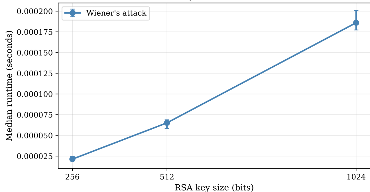
Wiener's Attack: Runtime vs. Key Size (median of 50 trials, error bars: IQR)
