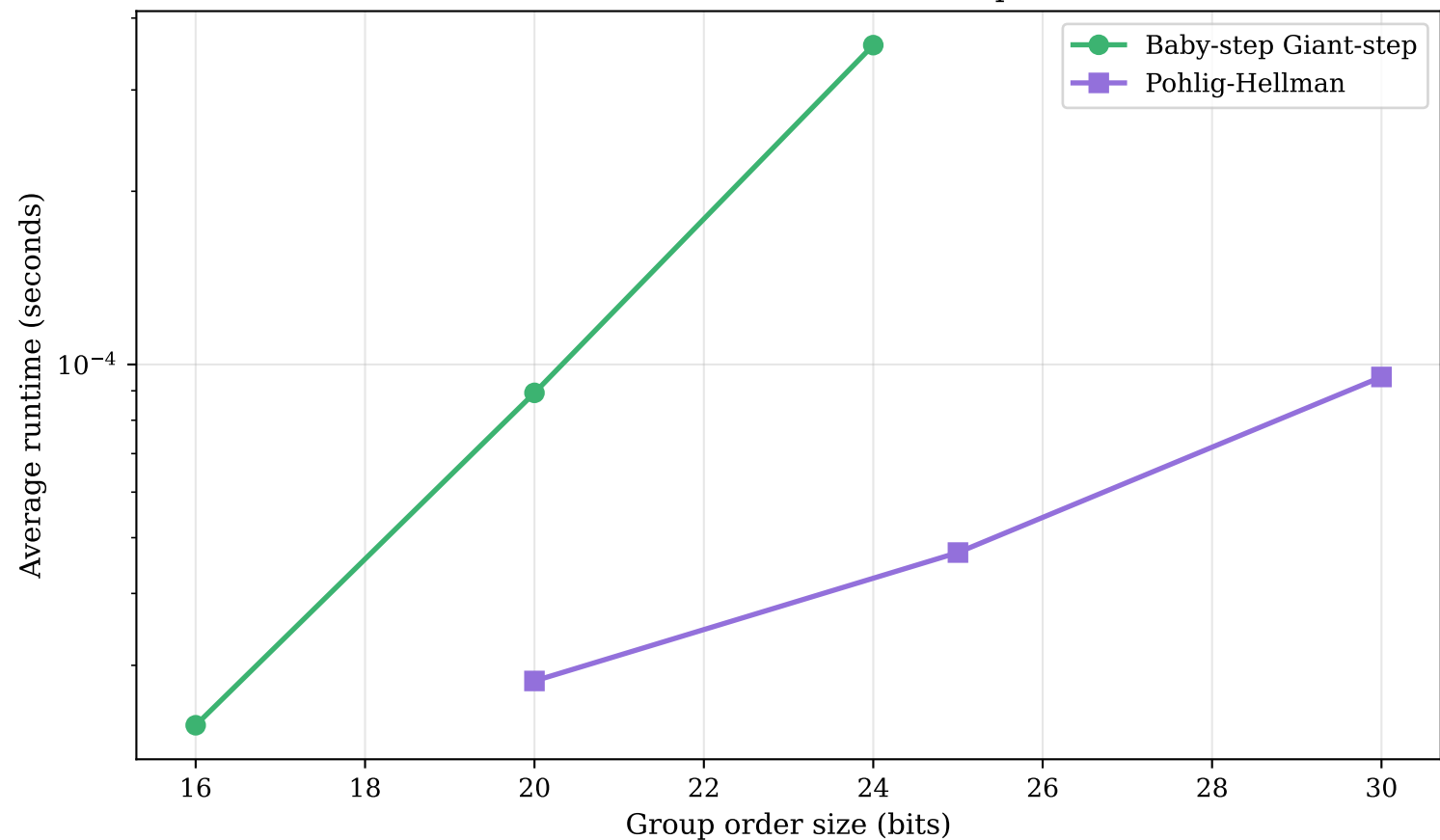
DH/ElGamal Attack Runtime Comparison
