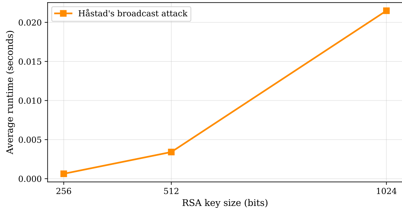
Håstad's Broadcast Attack: Runtime vs. Key Size (5 trials each)
