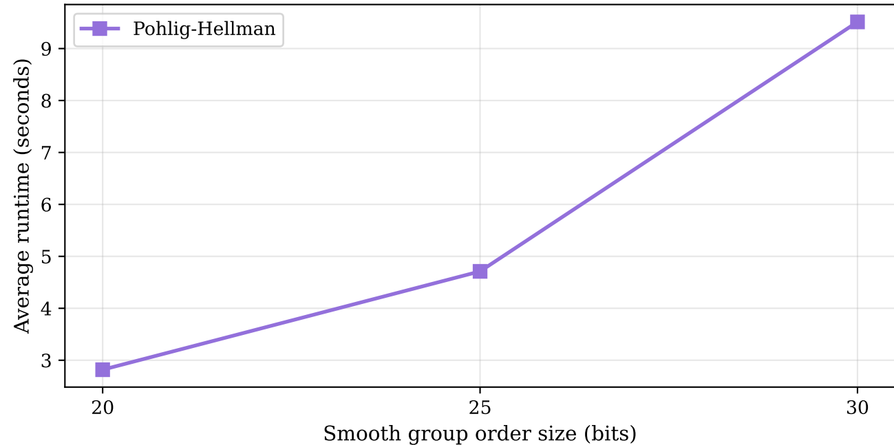
1e-5 Pohlig-Hellman: Runtime vs. Group Order Size (5 trials each)
