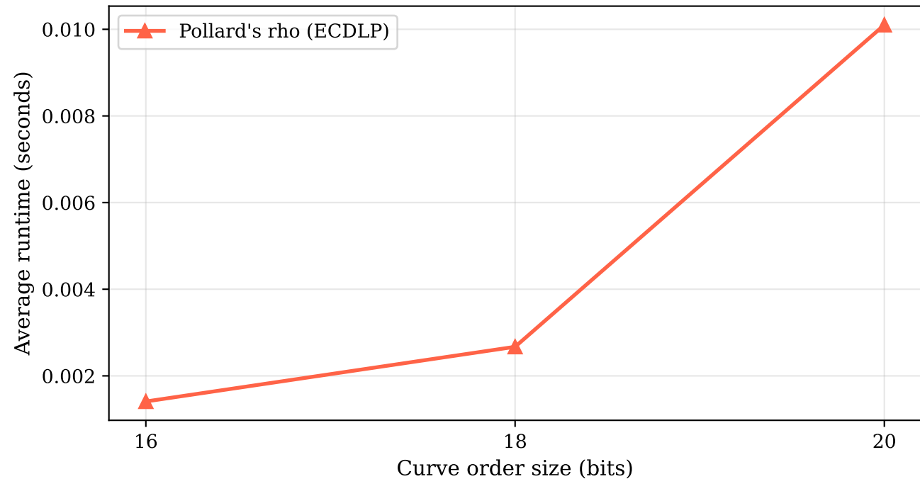
Pollard's Rho (ECDLP): Runtime vs. Curve Order Size (5 trials each)
