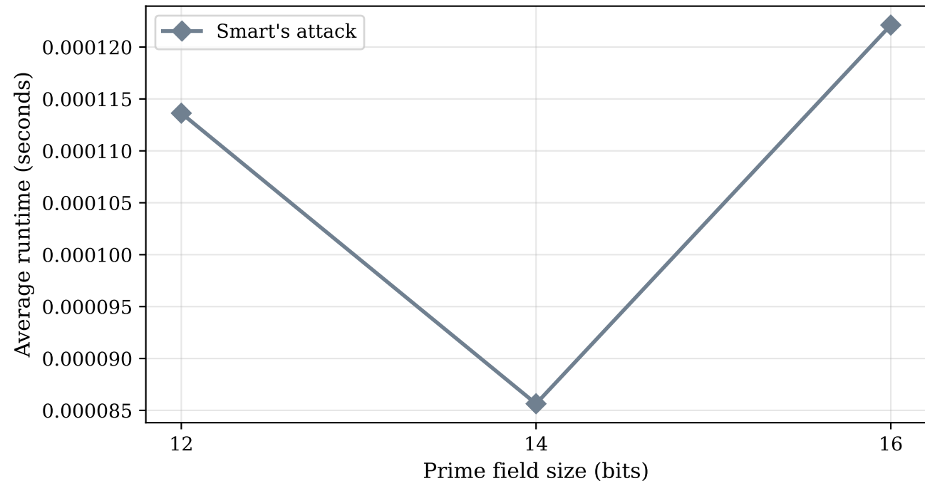
Smart's Attack: Runtime vs. Prime Field Size (5 trials each)
