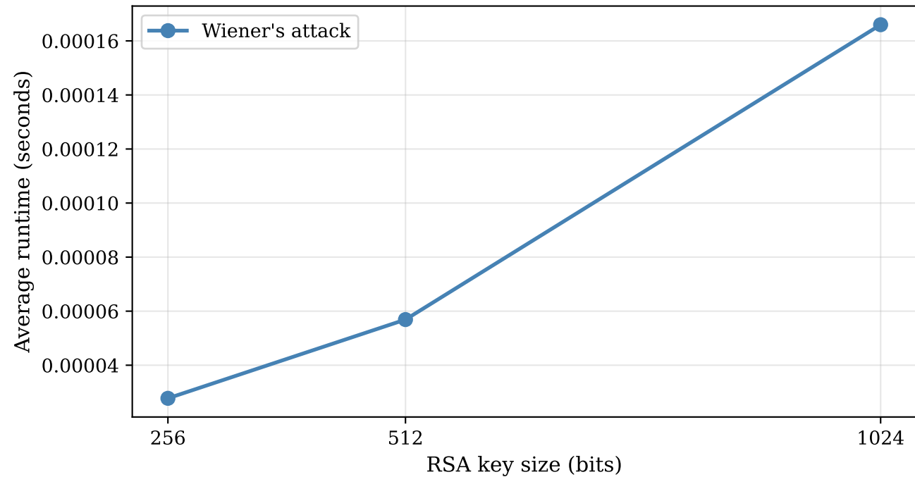
Wiener's Attack: Runtime vs. Key Size (5 trials each)
