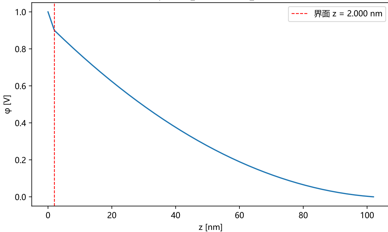
MOS 耗尽冒烟: \varphi(z) ( V_G = 1.0\text{ V} , N_A = 1\text{e}17\text{ cm}^{-3} )
