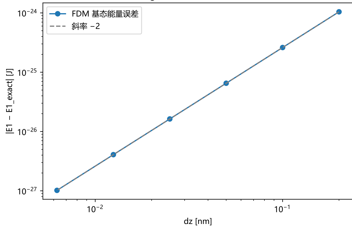
Schrödinger-FDM 收敛阶 (无限阱基态)
