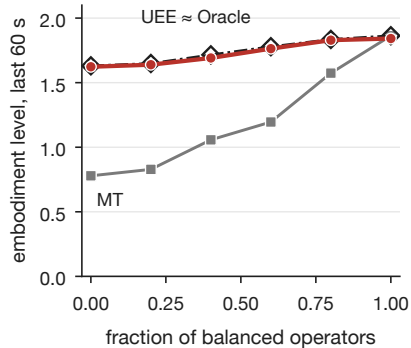
A Benefit depends on population variety
