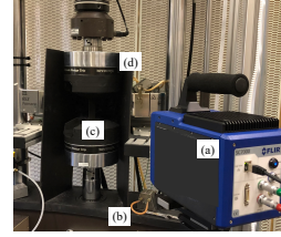
図.2: Equipment used in infrared stress measurement.
