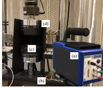
図.2: Equipment used in infrared stress measurement.
