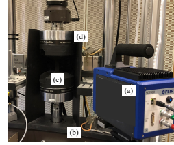
図.2: Equipment used in infrared stress measurement.
