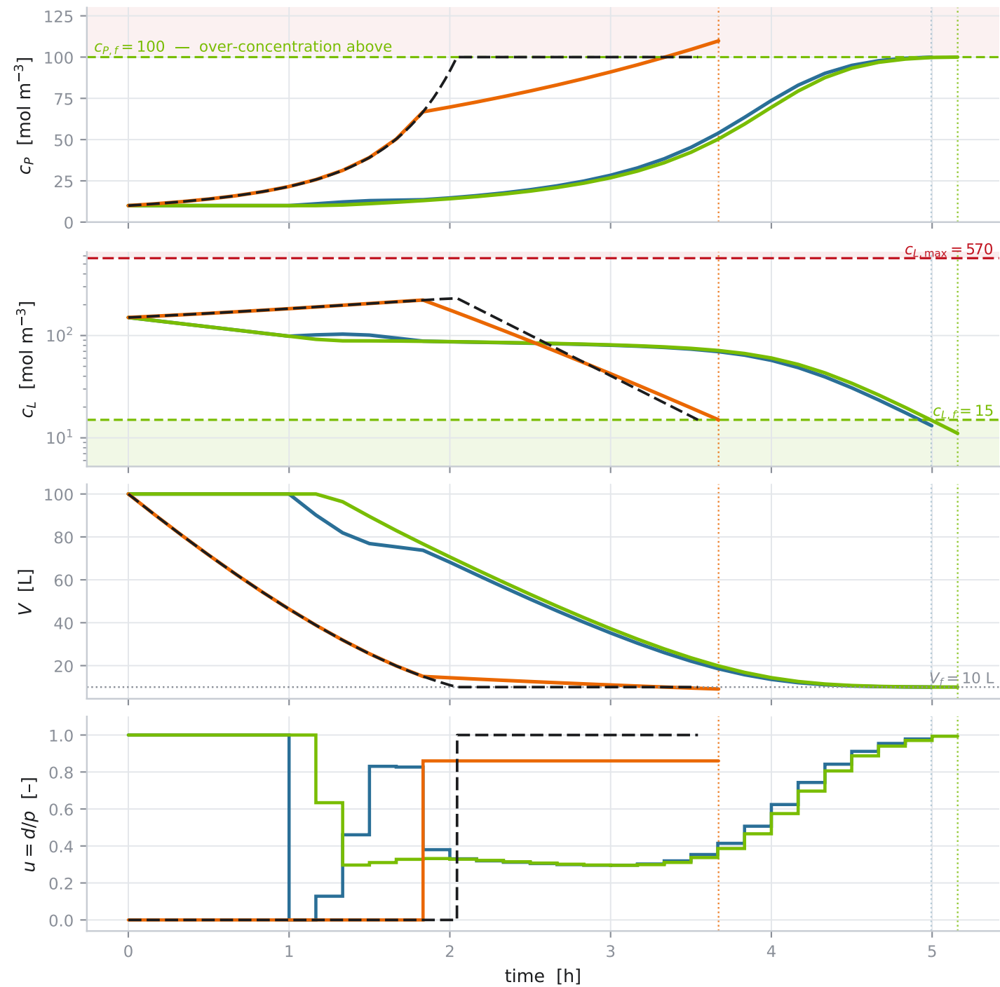
Task 3 — Eq. (3) vs. the heuristic policy of Eq. (4)
