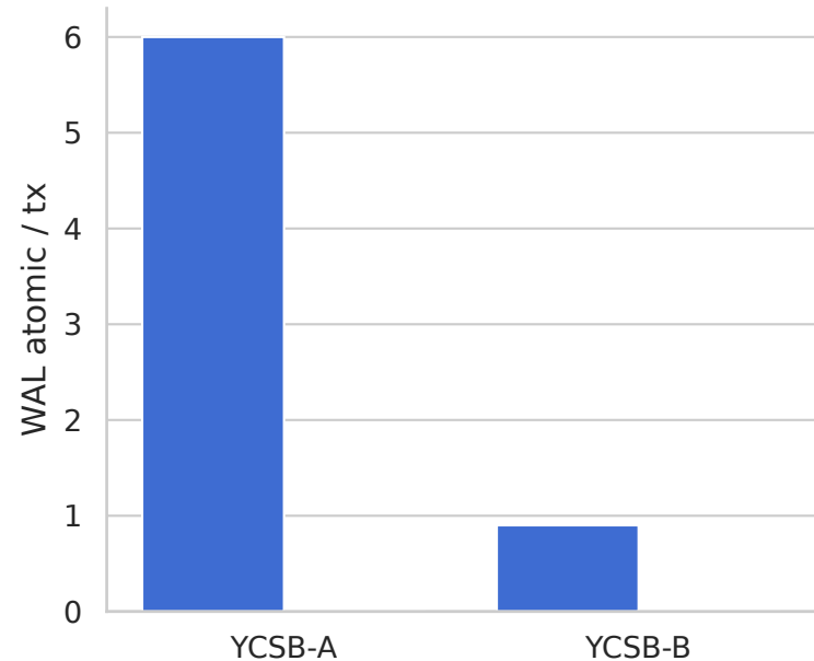
global atomic allocation
