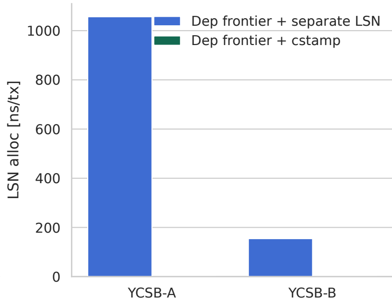
WAL-side LSN allocation
