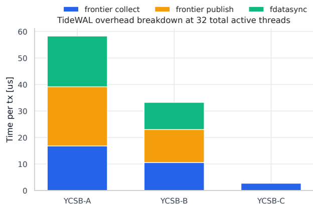
図 8 TideWAL overhead breakdown.
