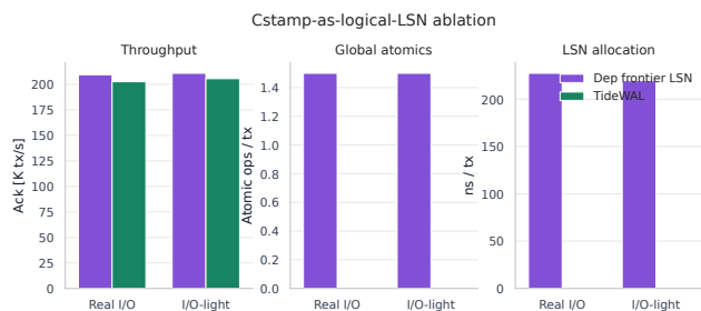
図 7 Cstamp-as-logical-LSN ablation.
