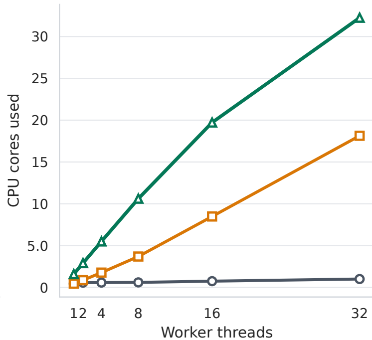
CPU cores
