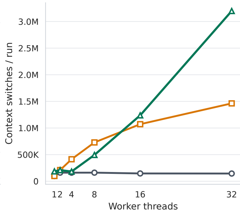
Context switches
