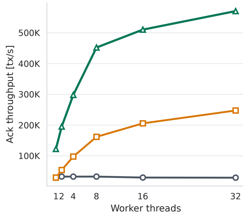
Throughput
