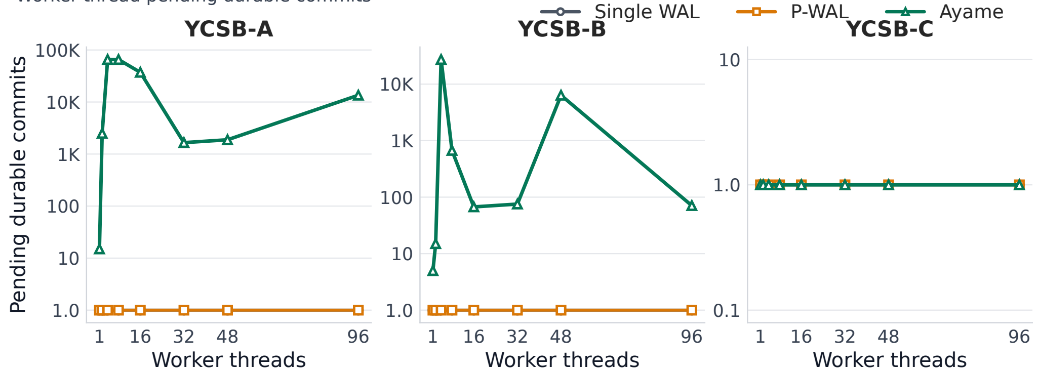
Worker-thread pending durable commits
