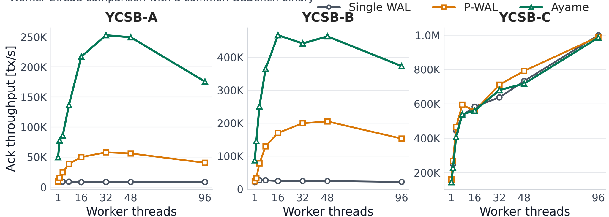
Worker-thread comparison with a common CCBench binary
