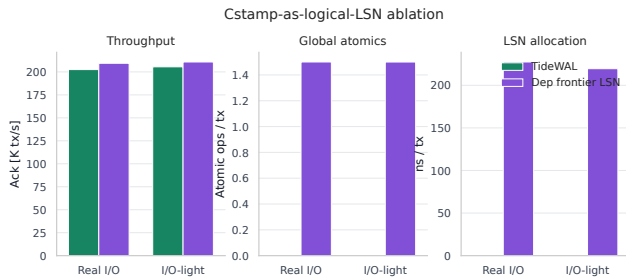
図 7 Cstamp-as-logical-LSN ablation.
