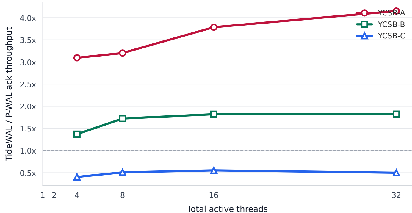
Fair total-thread-budget speedup with read-only WAL skip enabled for all systems
