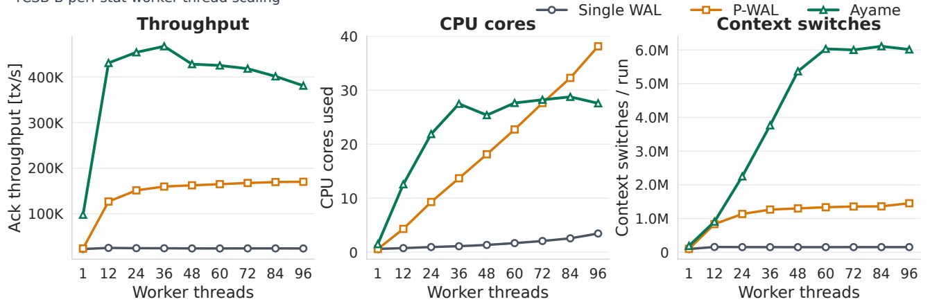
Fig. 11 Perf-stat summary for YCSB-B worker scaling.
