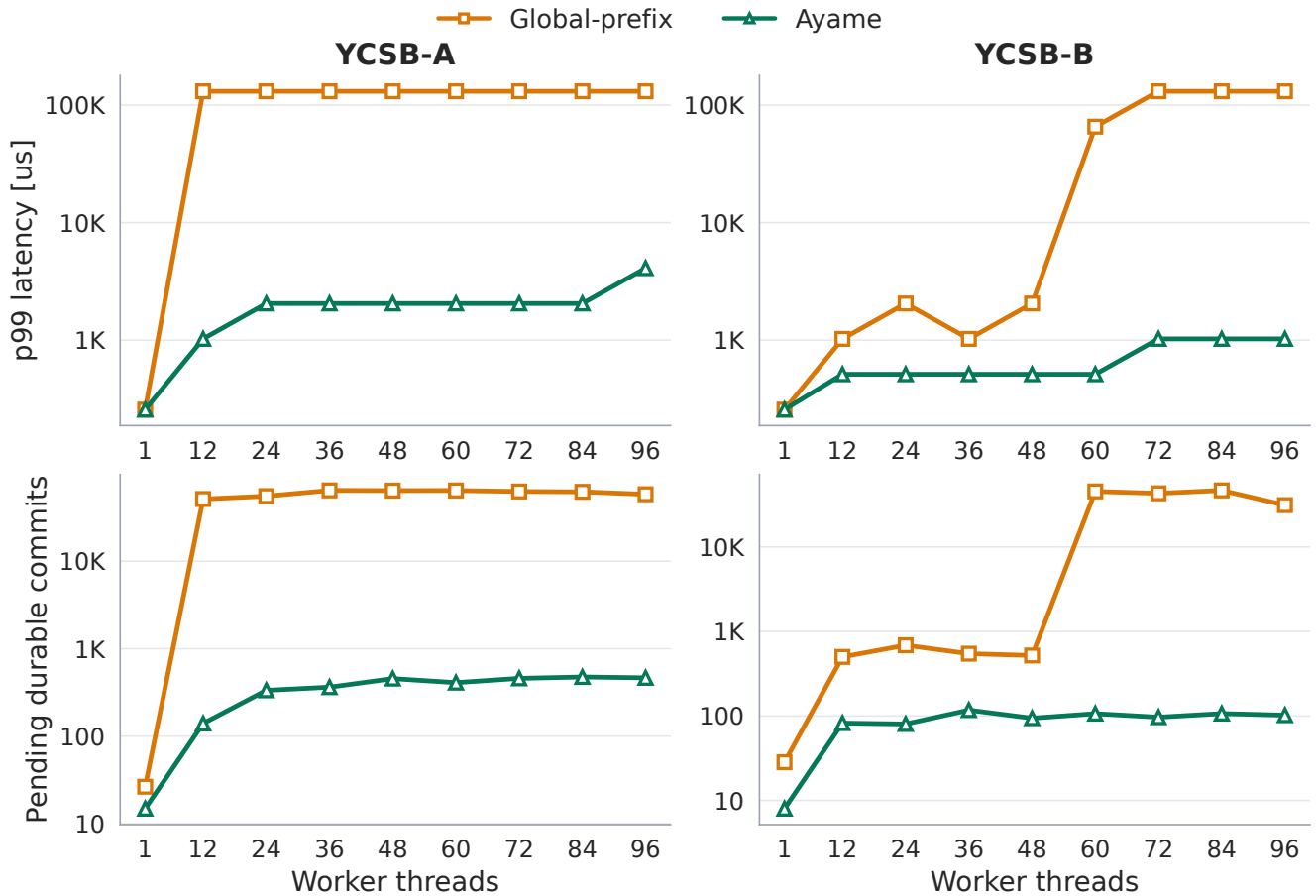
Fig. 7 Acknowledgment-policy comparison. Both variants use the same asynchronous WAL pipeline and differ only in the acknowledgment condition. The global-prefix rule keeps the pending count and p99 acknowledgment latency saturated on YCSB-A across the whole sweep, while the dependency-frontier rule keeps them bounded at every worker count.
