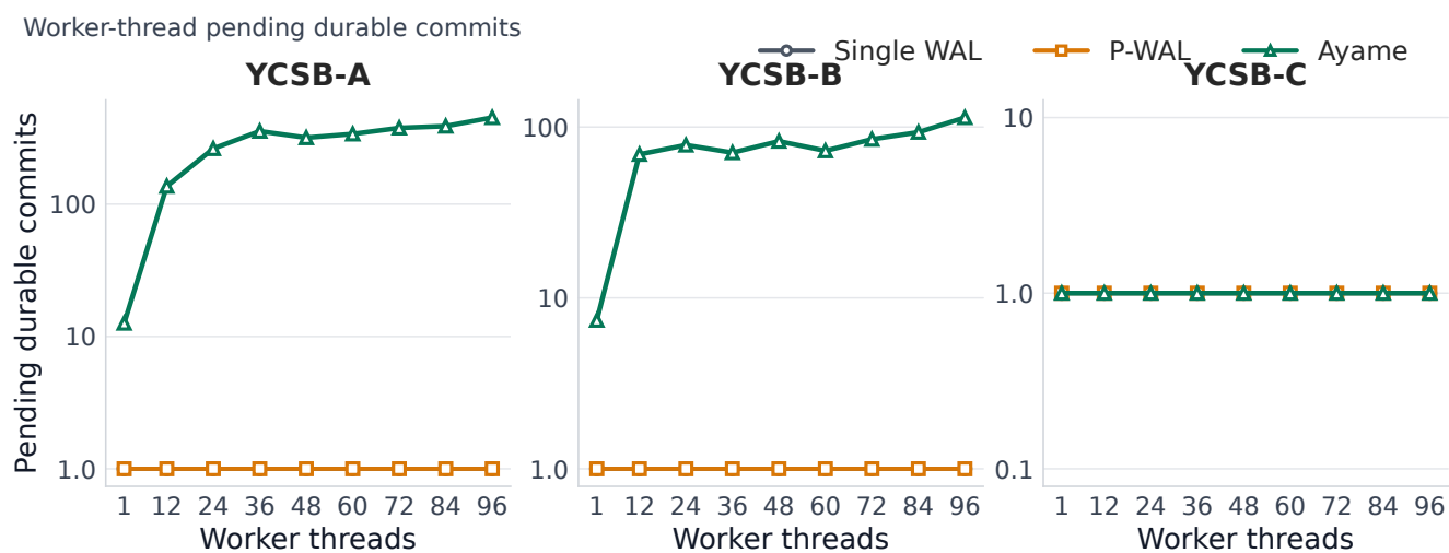
Fig. 5 Pending durable commits by transaction worker threads (log scale). Single WAL and P-WAL are synchronous and keep no pending durable commits; they are drawn at the axis floor.
