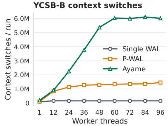
Fig. 10 Context-switch counts in the YCSB-B perf-stat worker-scaling runs.
