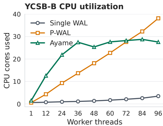
Fig. 9 CPU-core utilization in the YCSB-B perf-stat worker-scaling runs.
