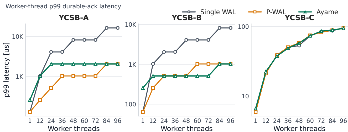
Fig. 4 P99 durable-acknowledgment latency by transaction worker threads.
