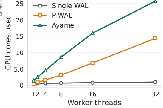
Fig. 8 CPU-core utilization in the YCSB-B perf-stat worker-scaling runs.
