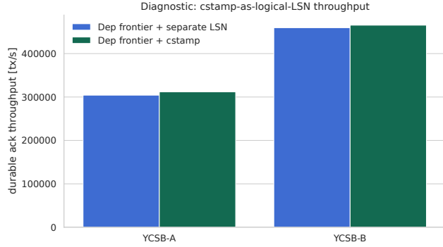
図 8 Diagnostic throughput results for commit-timestamp integration.
