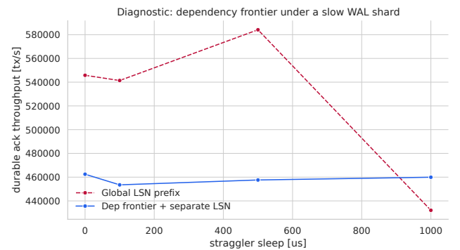
Figure 6 Diagnostic throughput results for dependency-frontier and straggler effects.
