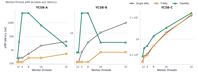
Figure 3 P99 durable-acknowledgment latency by transaction worker threads.
