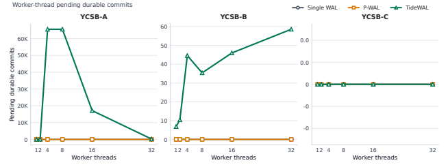
Figure 4 Pending durable commits by transaction worker threads.
