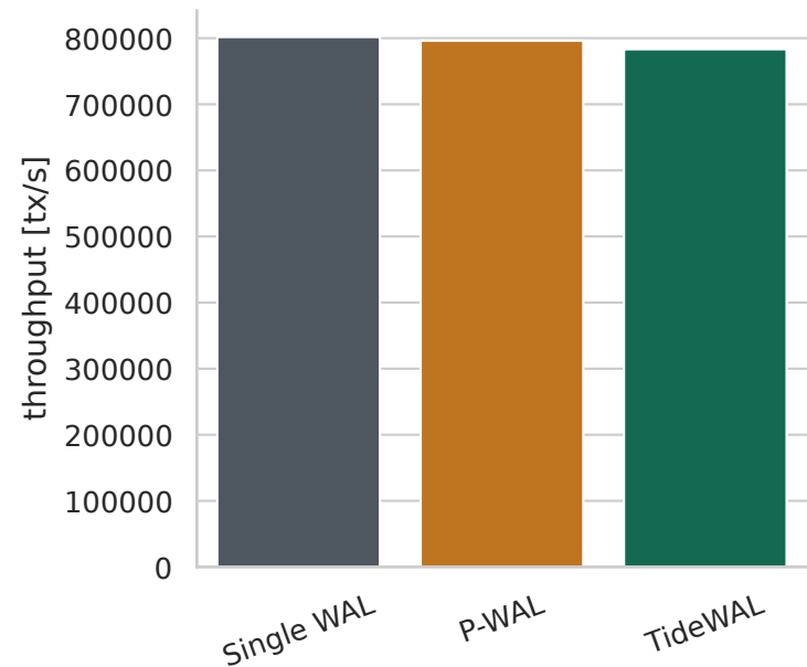
YCSB-C throughput
