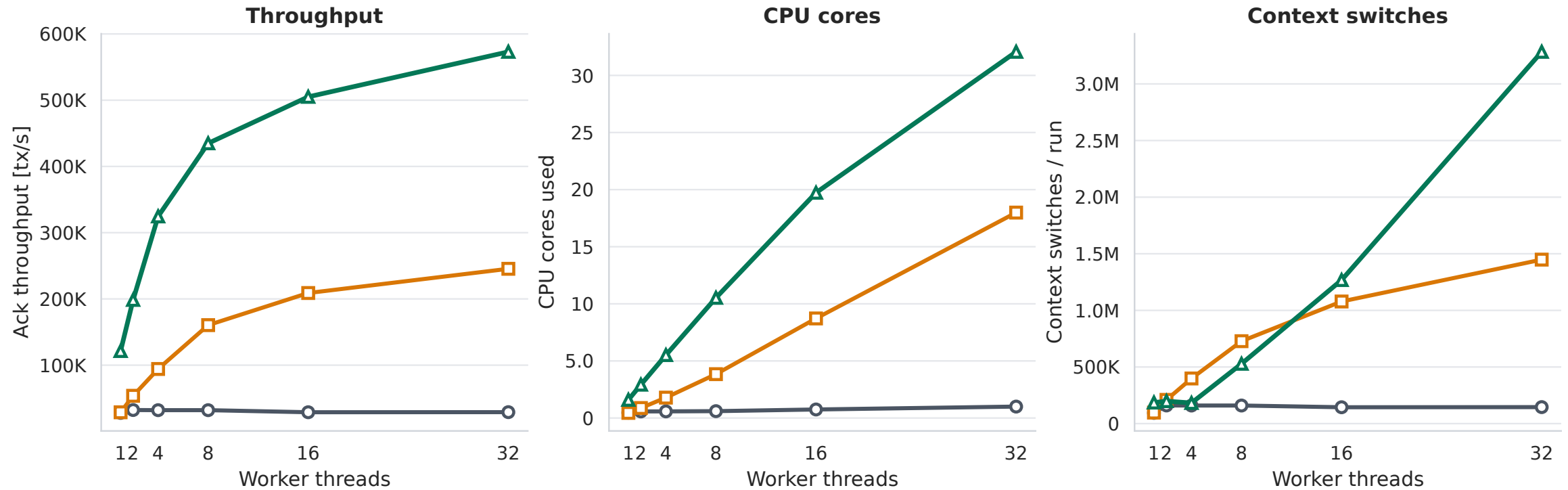
YCSB-B perf stat worker-thread scaling
