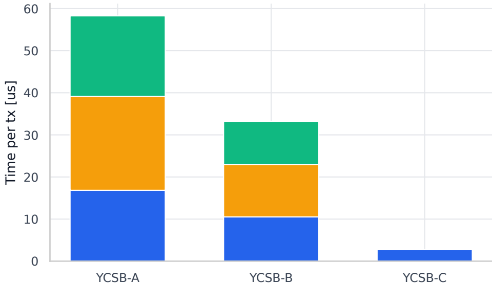
frontier collect frontier publish fdatsync TideWAL overhead breakdown at 32 total active threads
