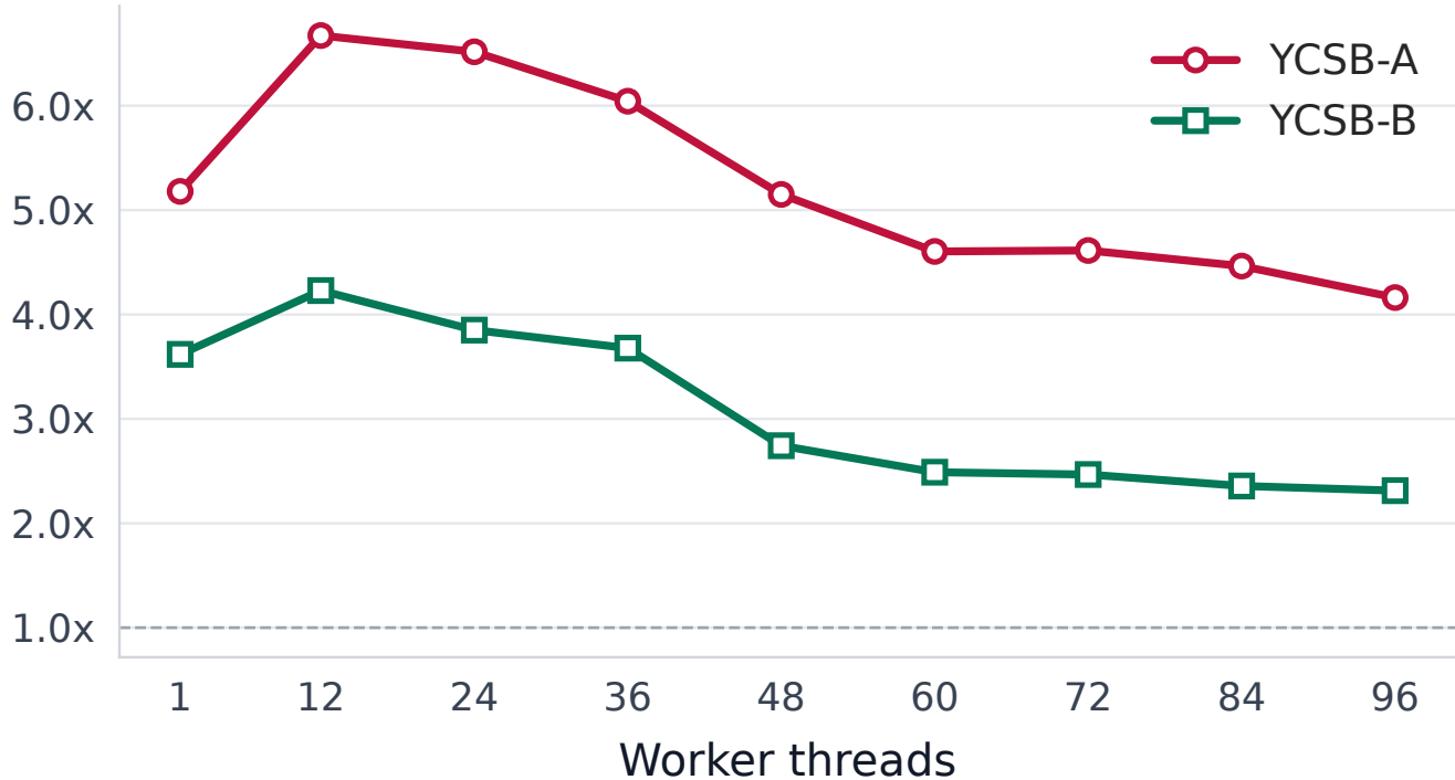
Worker-thread scaling; all modes use the same CCBench binary
