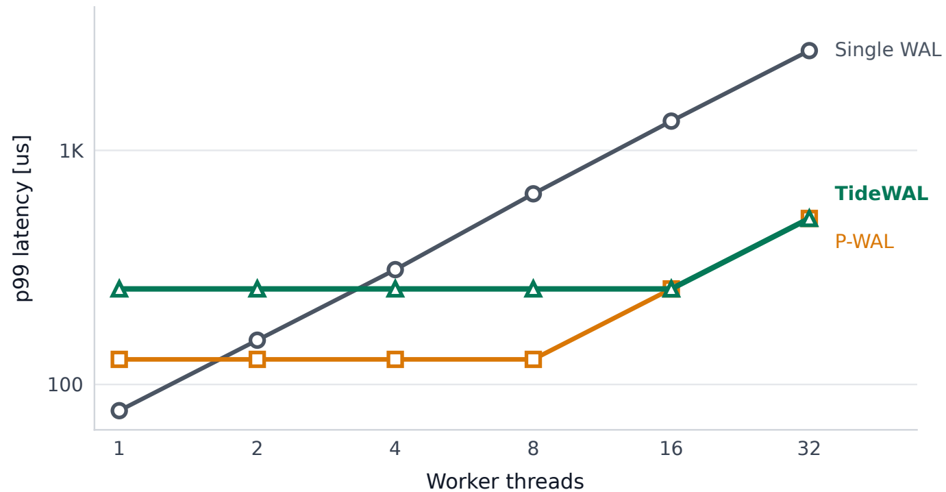
YCSB-B, p99 durable-ack latency; no confidence band
