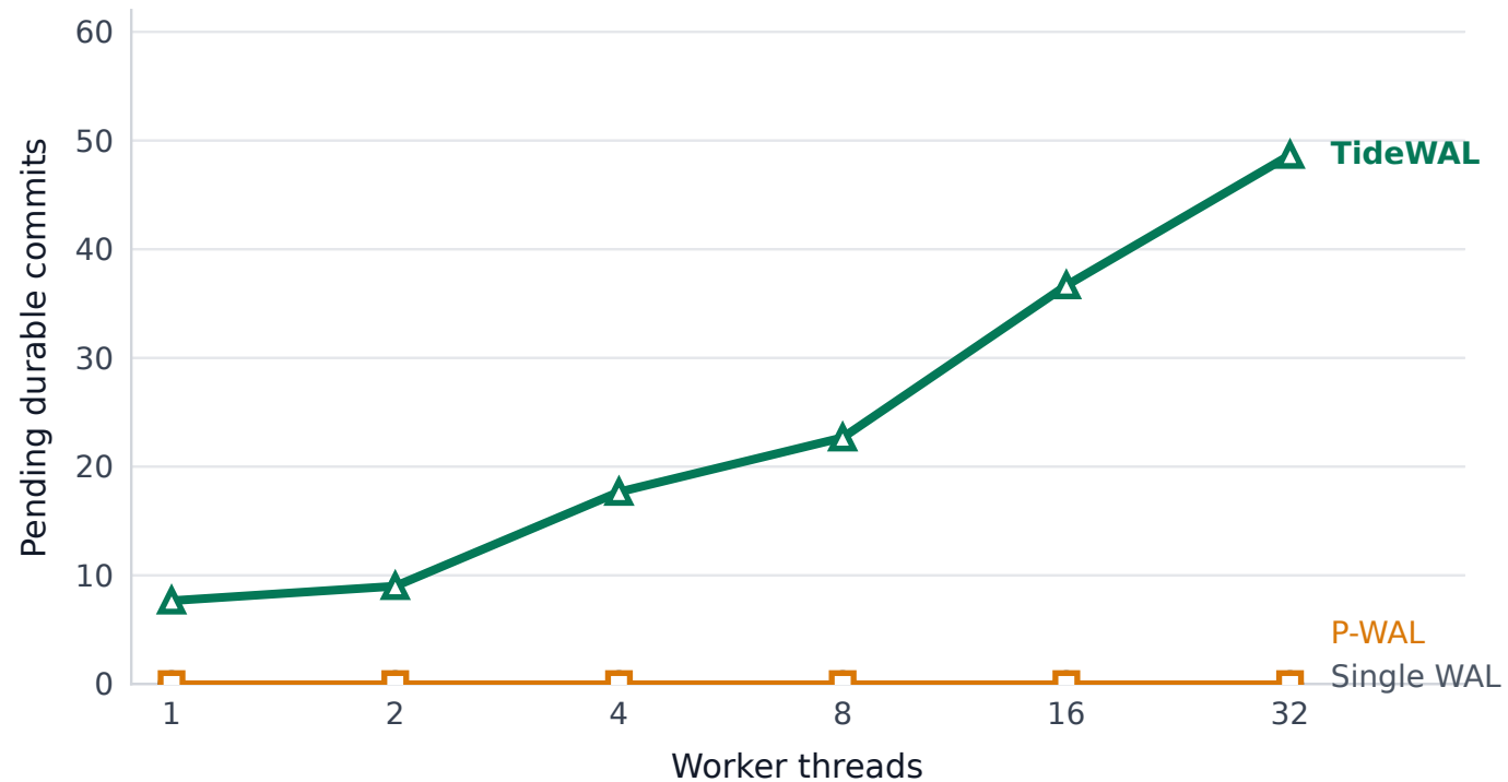
YCSB-B, measured at the end of the steady-state window
